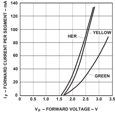
Figure 10. Forward Current vs. Forward Voltage.
